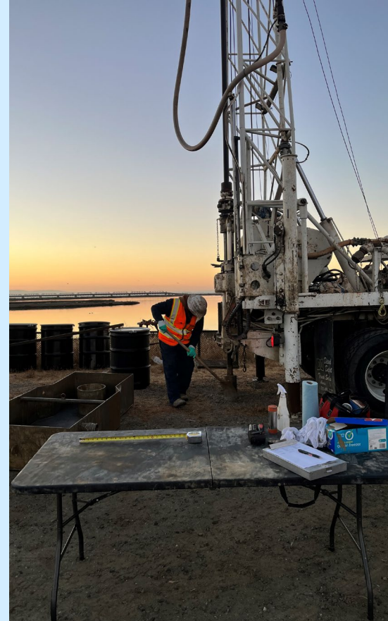
Geotechnical studies at Dumbarton Bridge Vista Point
